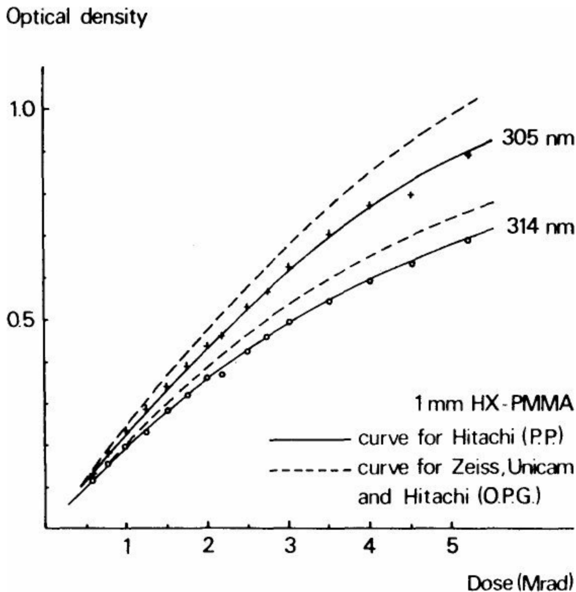
Figure 2. Difference in calibration curve of 1 mm HX Perspex™ measured on four different spectrophotometers. The same samples were measured on all four instruments.
