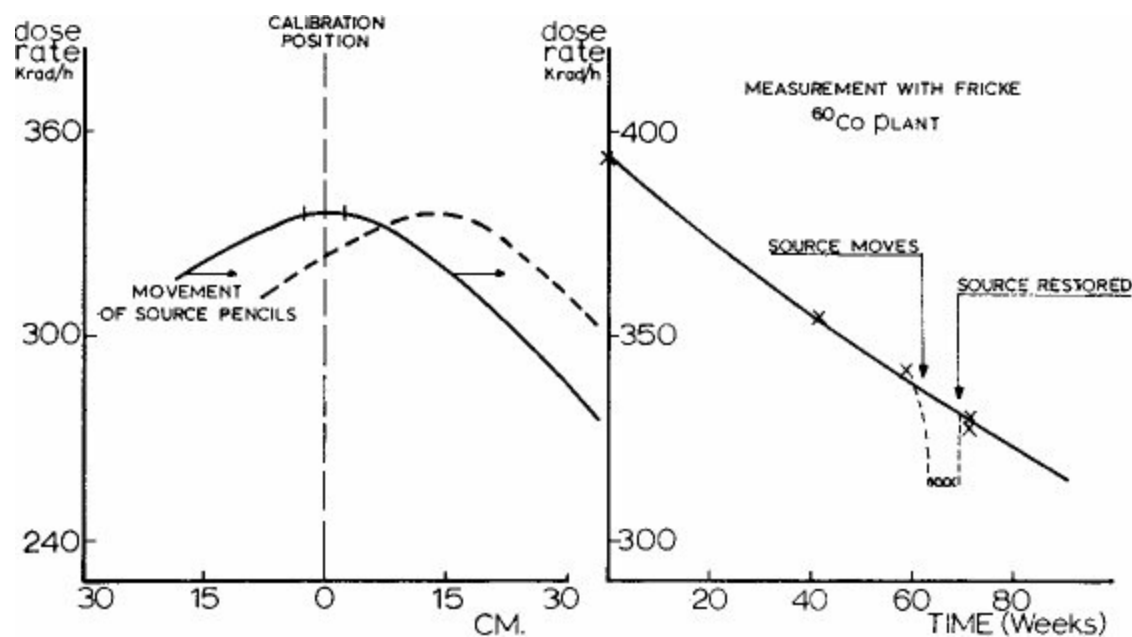
Figure 1. The effect of the movement of source pencils within the source frame on the dose rate at a calibration position in an industrial facility.
